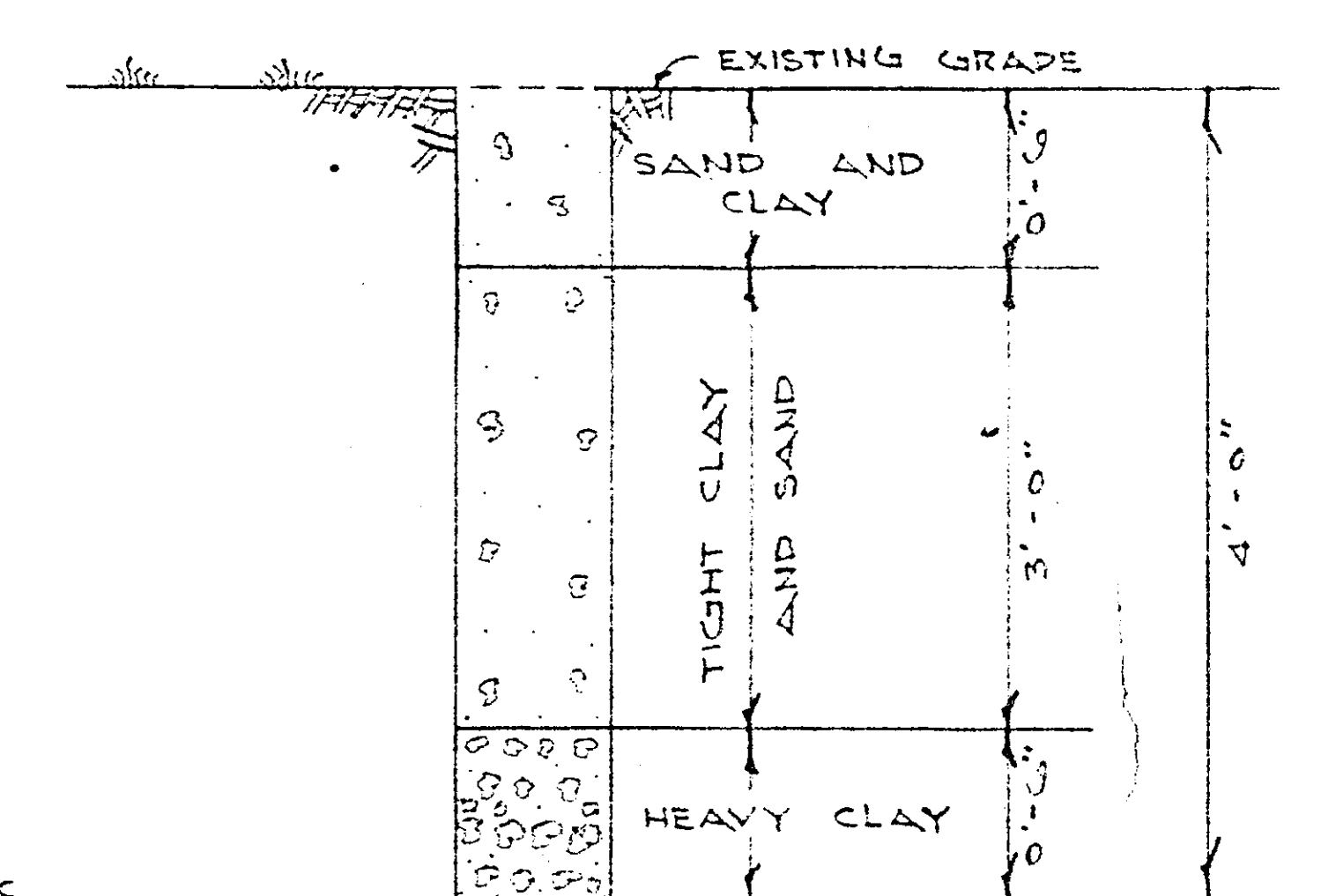
BORING NOT TO SCALE
