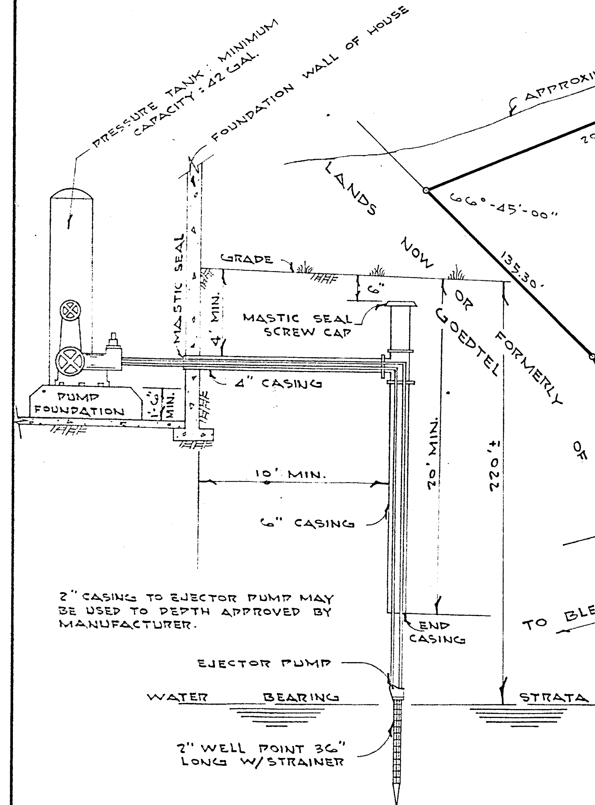
SKETCH OF DRILLED WELL NOT TO SCALE
