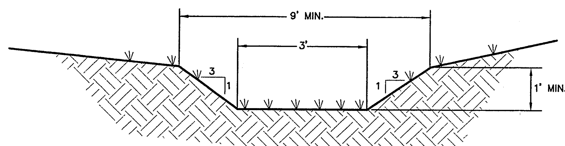
DRAINAGE SWALE DETAIL (DETAIL C) NOT TO SCALE
