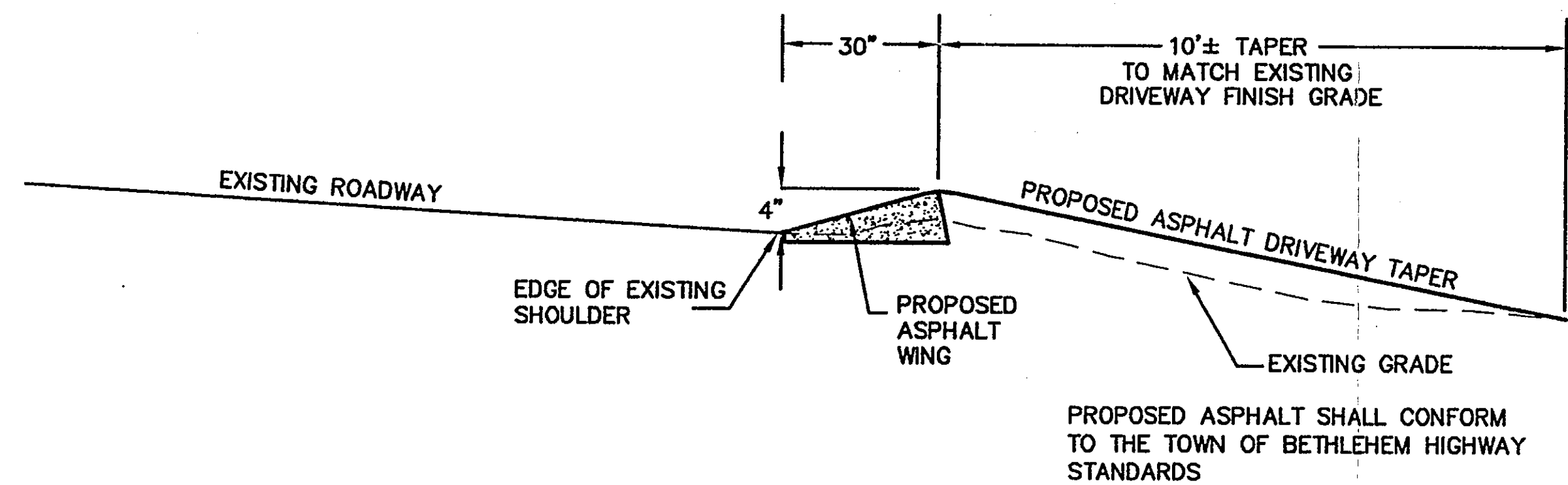
DRIVEWAY GUTTER DETAIL (DETAIL A) NOT TO SCALE
