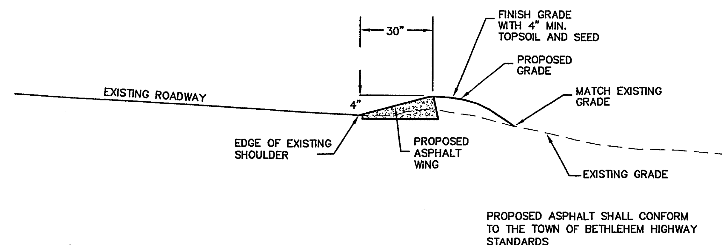
ASPHALT WING DETAIL (DETAIL B) NOT TO SCALE
