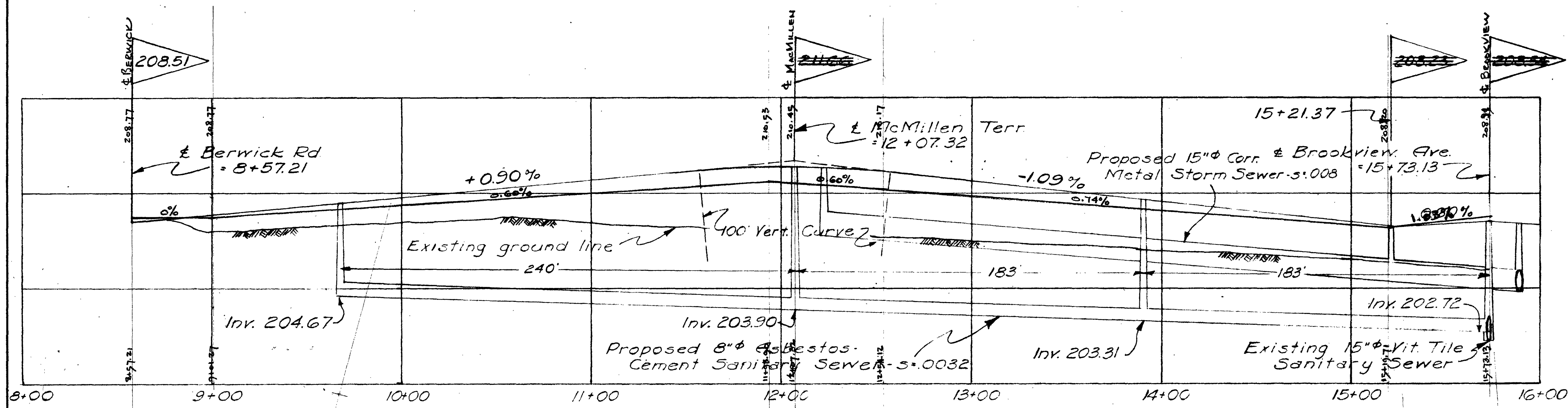
MONTROSE DRIVE Scales: Horizontal 1"=40' Vertical 1"=4'
