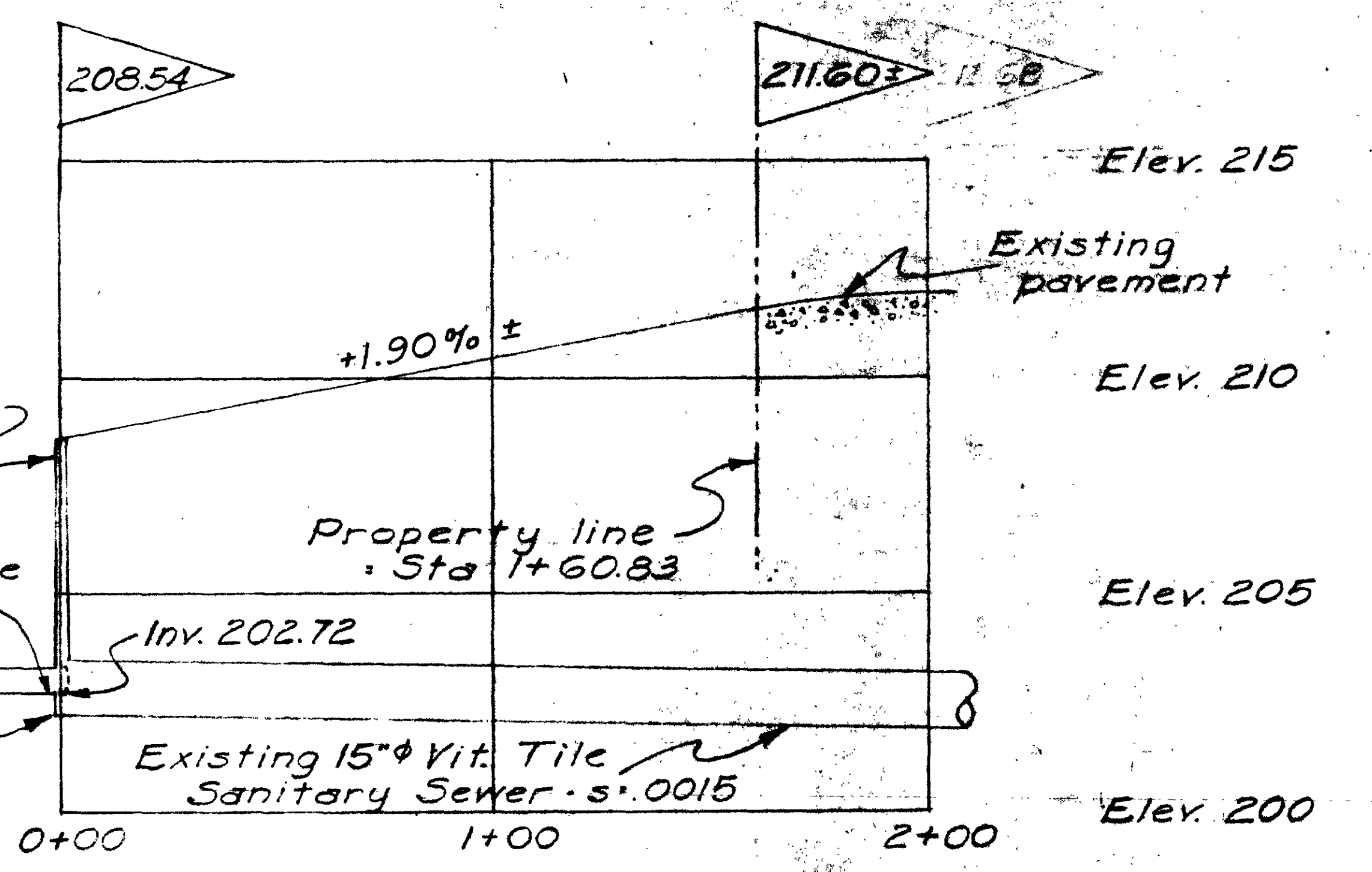
BROOKVIEW AVENUE Scales: Horizontal 1"=40' Vertical 1"=4'
