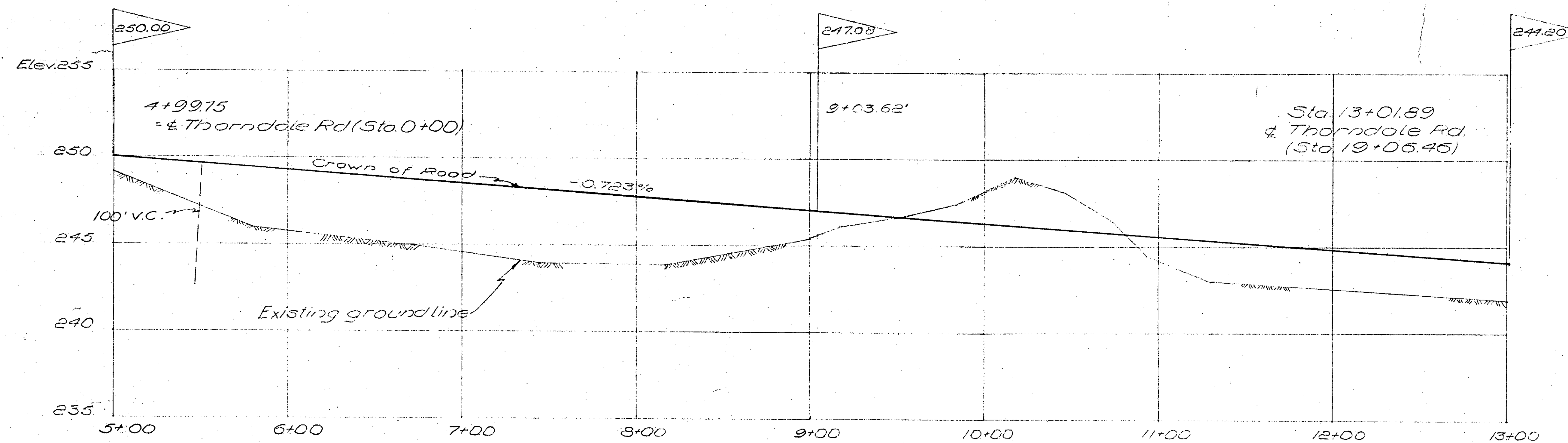
PROFILE of Portion of SOUTHWOOD DRIVE Scale: Horiz. 1"=50' Vert. 1"=5'
