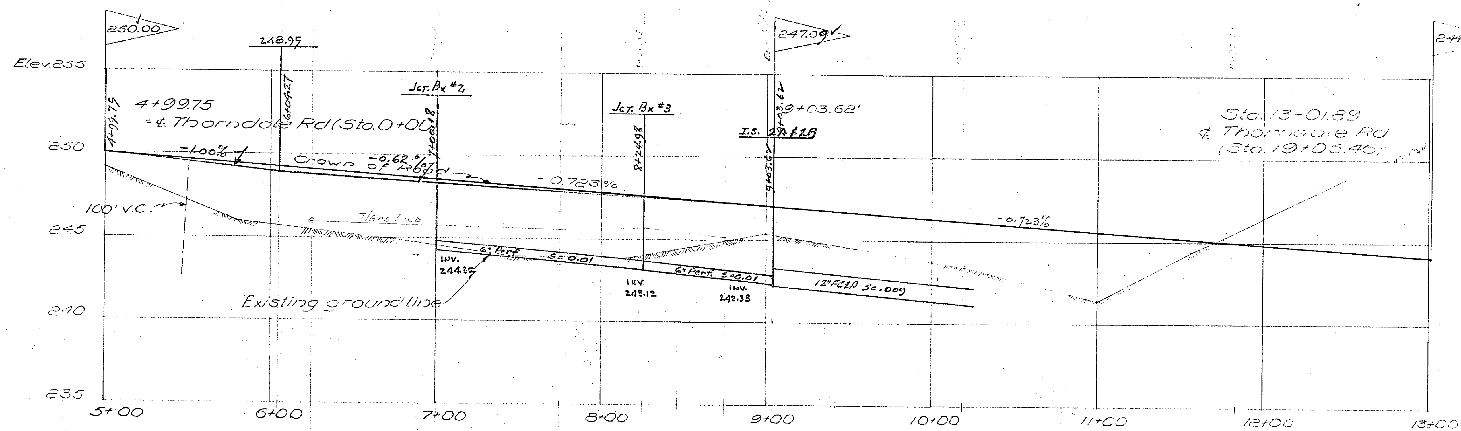
PROFILE of Portion of SOUTHWOOD DRIVE Scale: Horiz. 1"=50' Vert. 1"=5'
