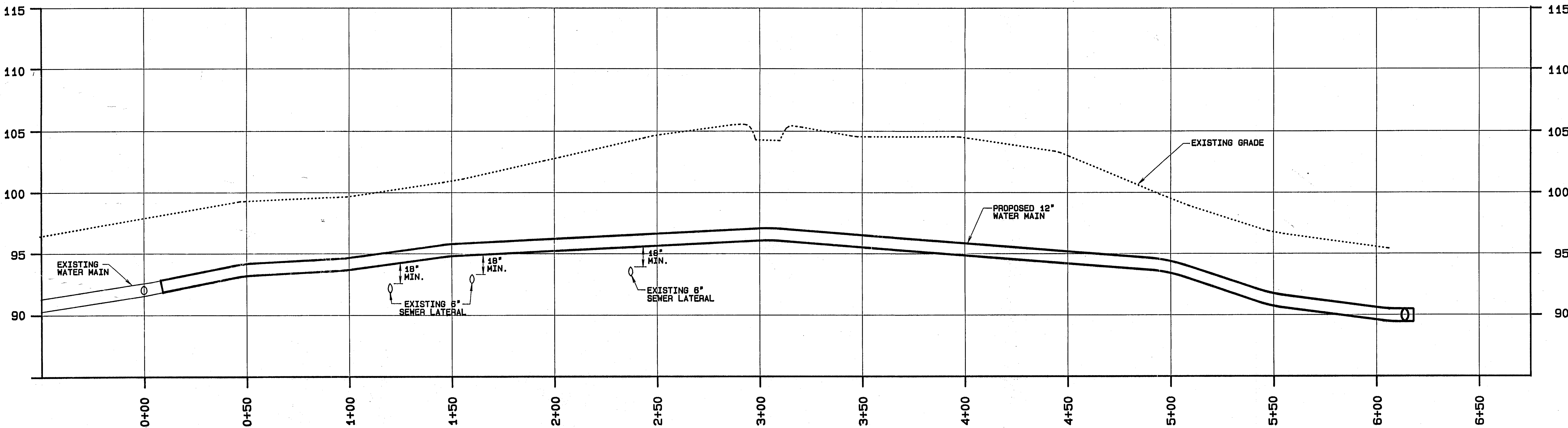
PROFILE PROPOSED WATER MAIN SCALE: HORIZONTAL 1"=30' VERTICAL 1"=5'
