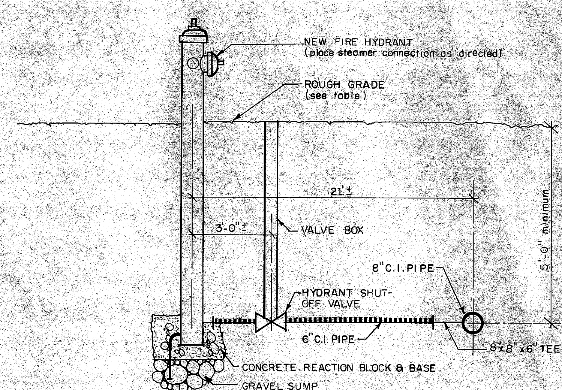
DETAIL "I" new fire hydrants
