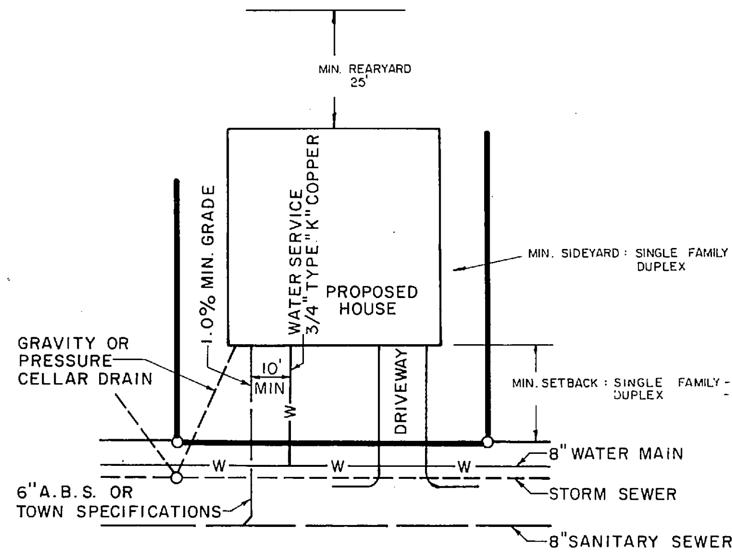
TYPICAL LOT LAYOUT (NOT TO SCALE)
