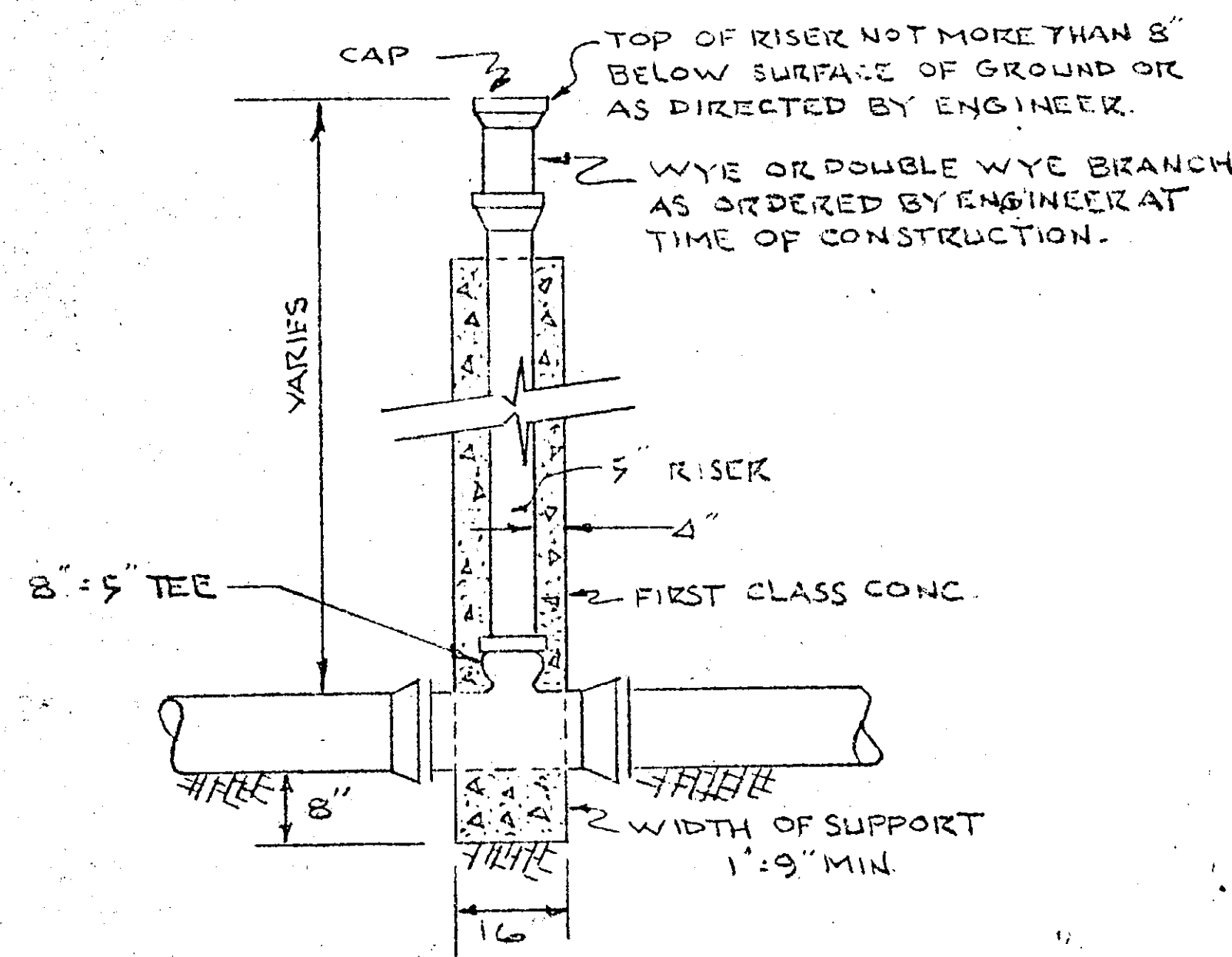
DETAIL OF VERTICAL PIPE RISER (NOT TO SCALE)
