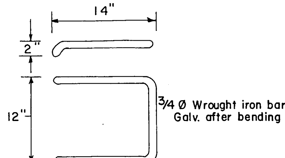
MANHOLE STEPS (Not to Scale)
