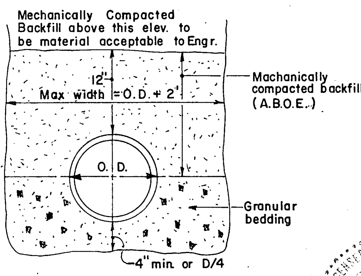
SEWER PIPE TRENCH DETAILS (Not to Scale)
