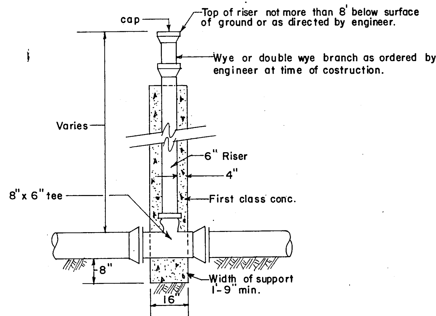
DETAIL OF VERTICAL PIPE RISER (Not to Scale)
