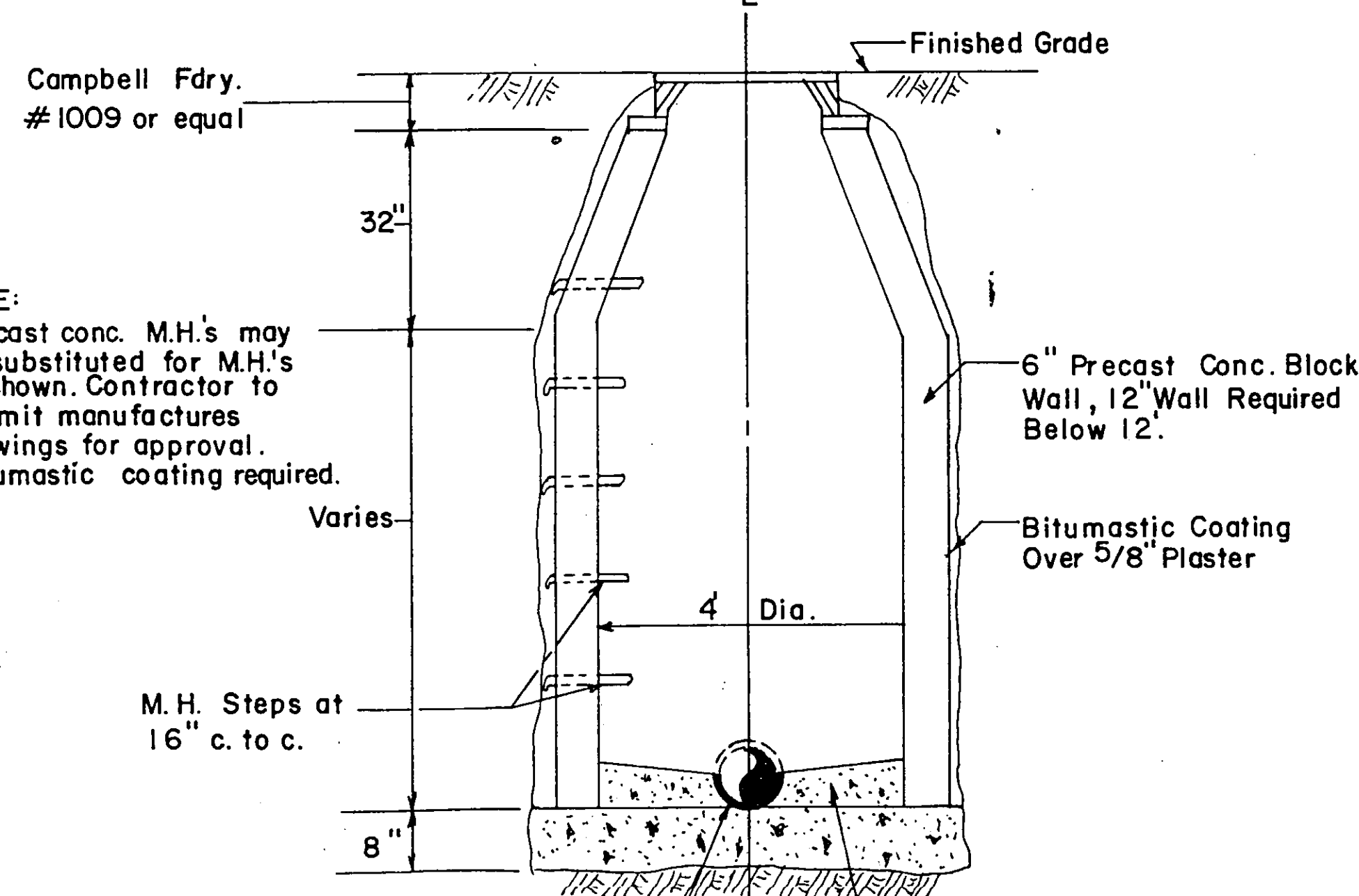
STANDARD MAN HOLE (Not to Scale)
