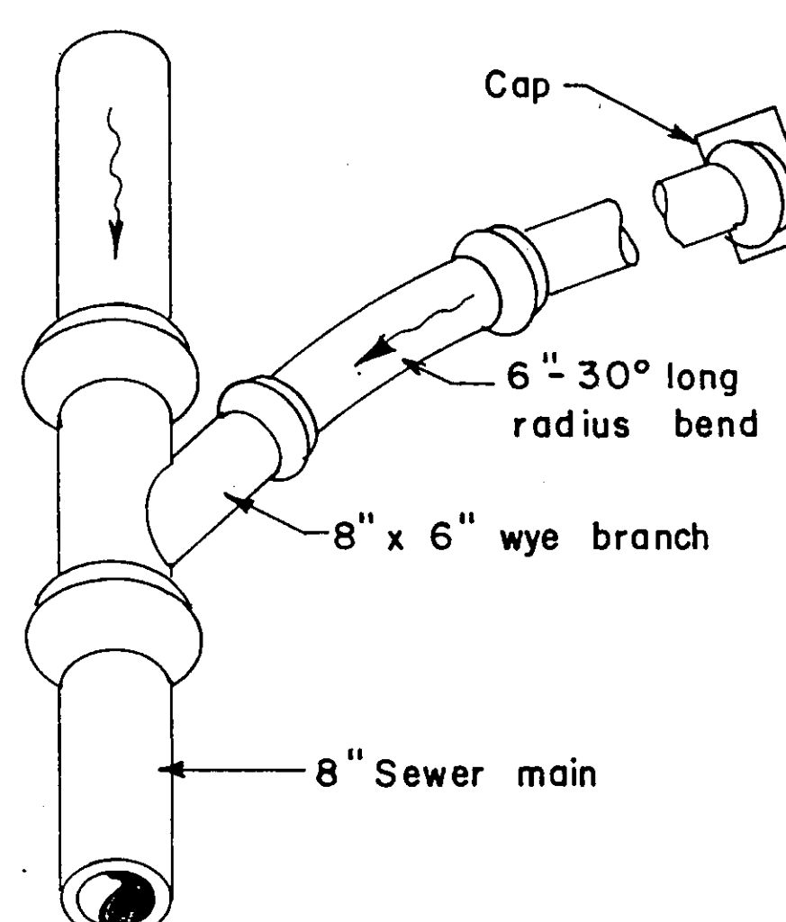
DETAIL OF LATERAL CONNECTION (Not to Scale)
