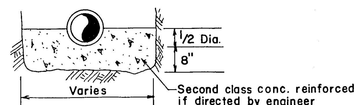
CONCRETE PIPE CRADLE (Not to Scale)
