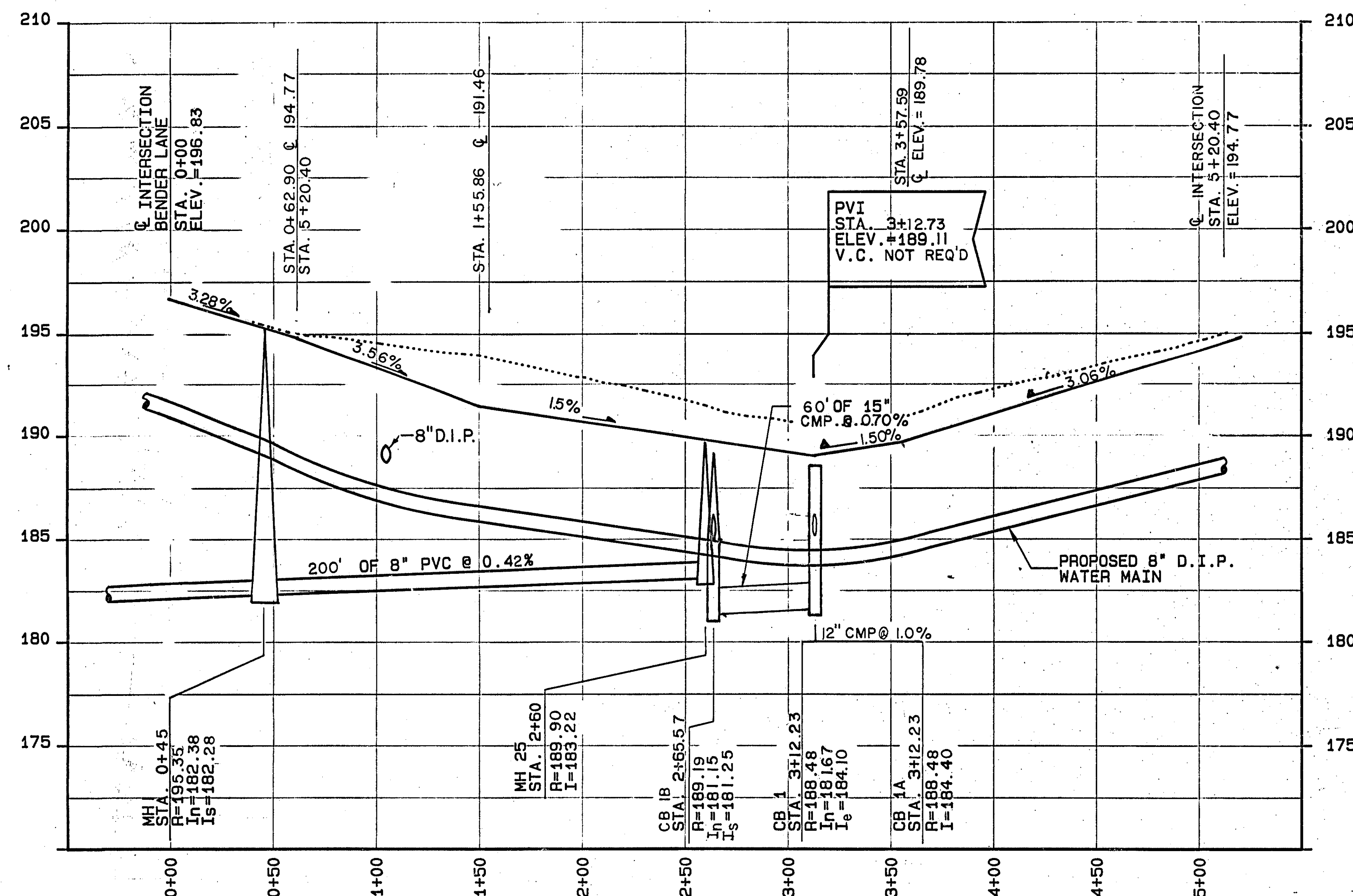
\bar{C} PROFILE - FOXFIRE LANE
