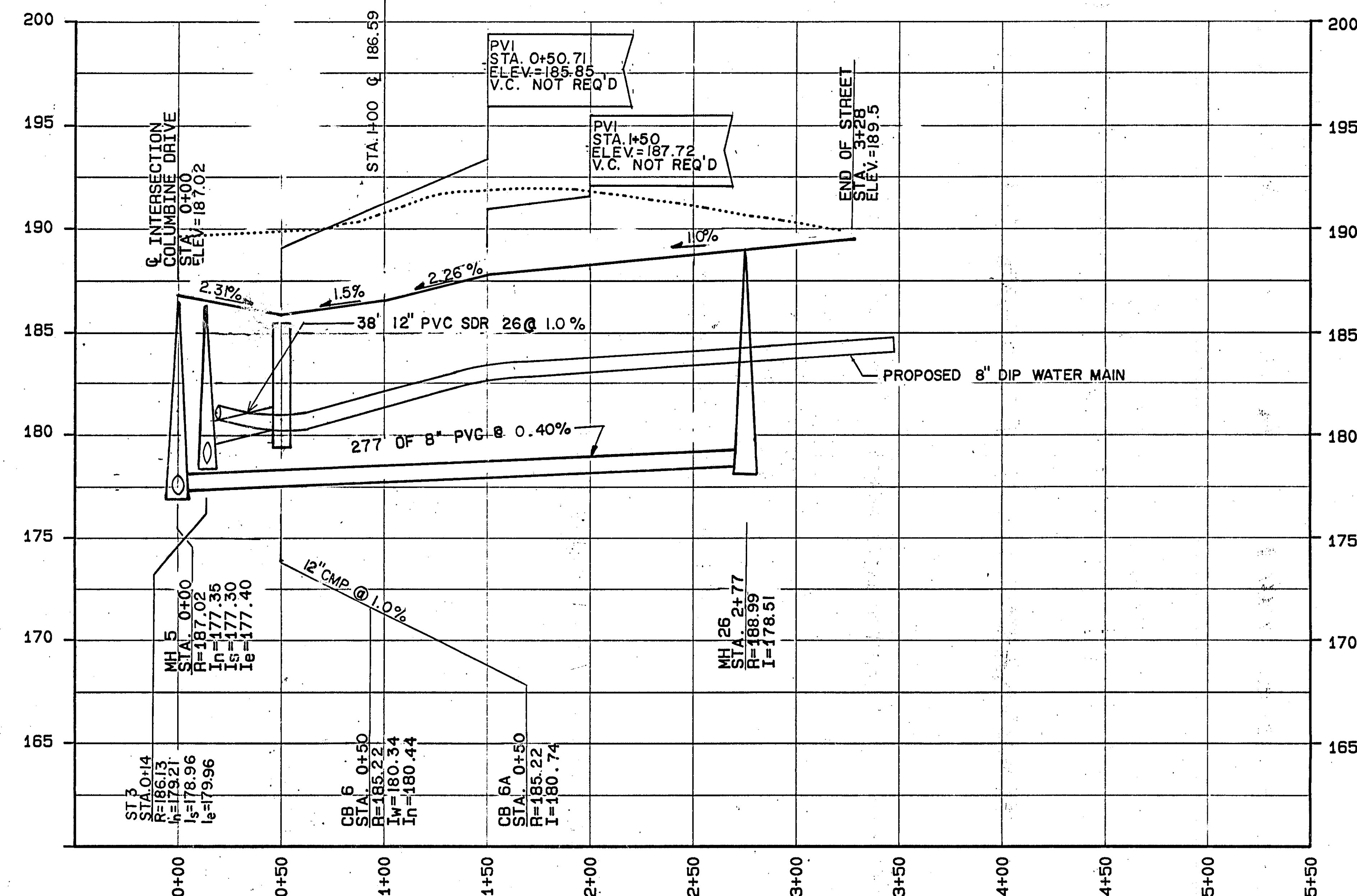
PROFILE OF \bar{C} THISTLE LANE
