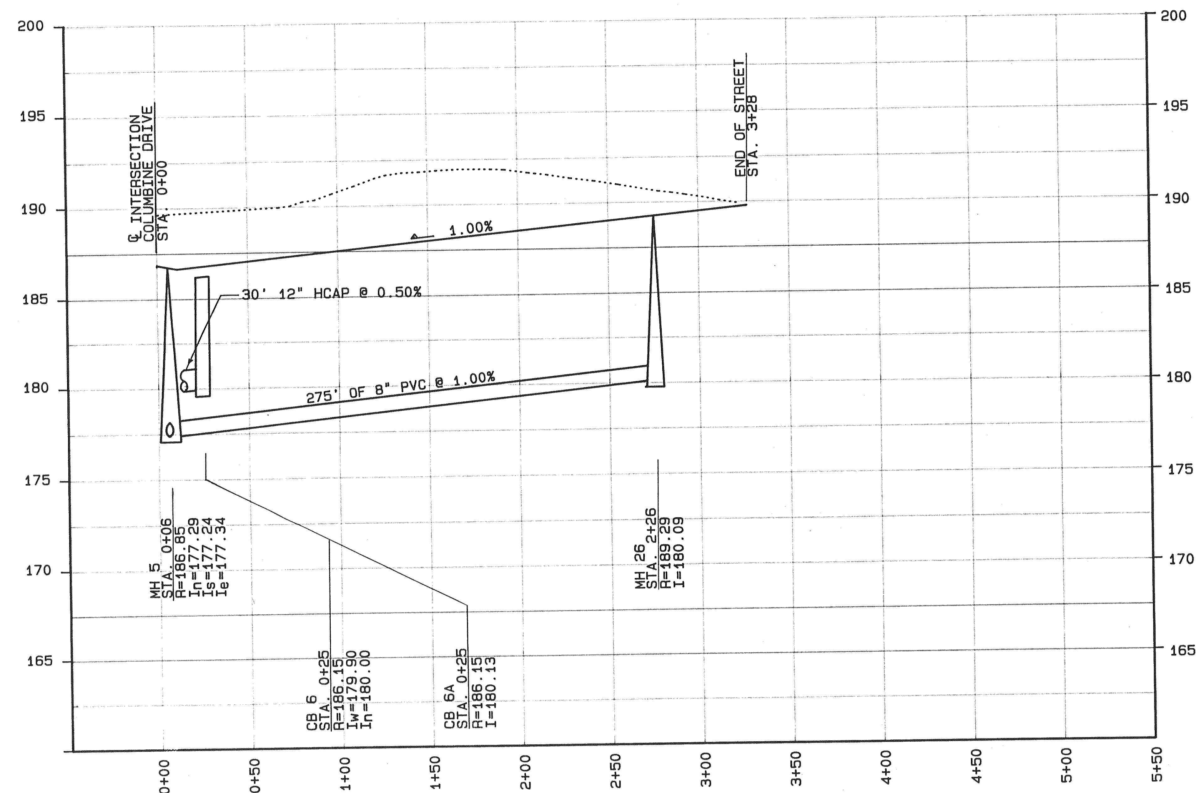
PROFILE OF Q THISTLE LANE
