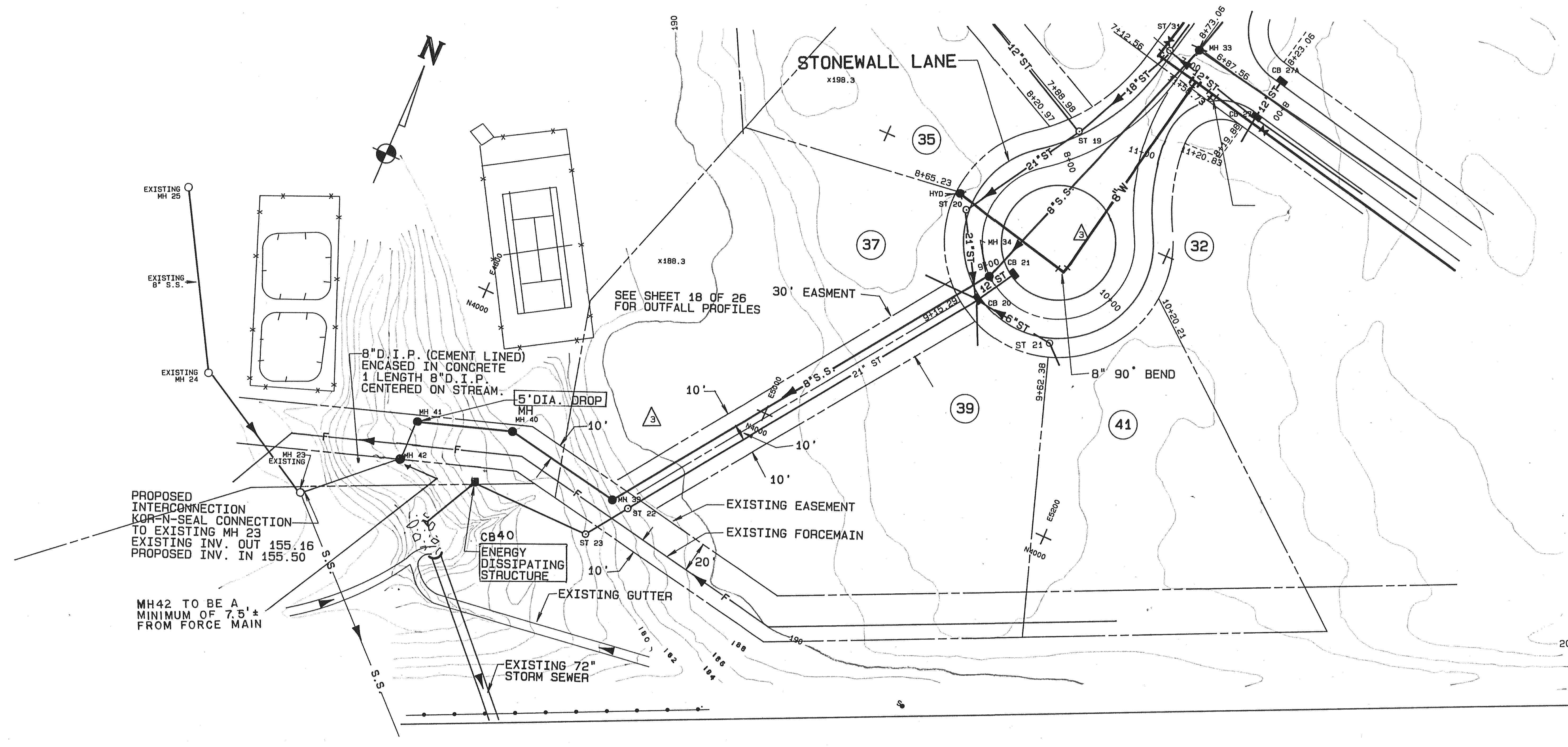
PLAN - STONEWALL LANE UTILITY OUTFALLS
