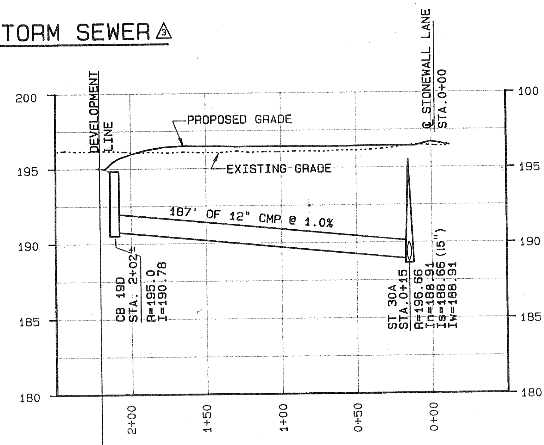
PROFILE-NORTH WINDSOR COURT DRAINAGE SCALE: HORIZ. 1"=50' VERT. 1"=5'
