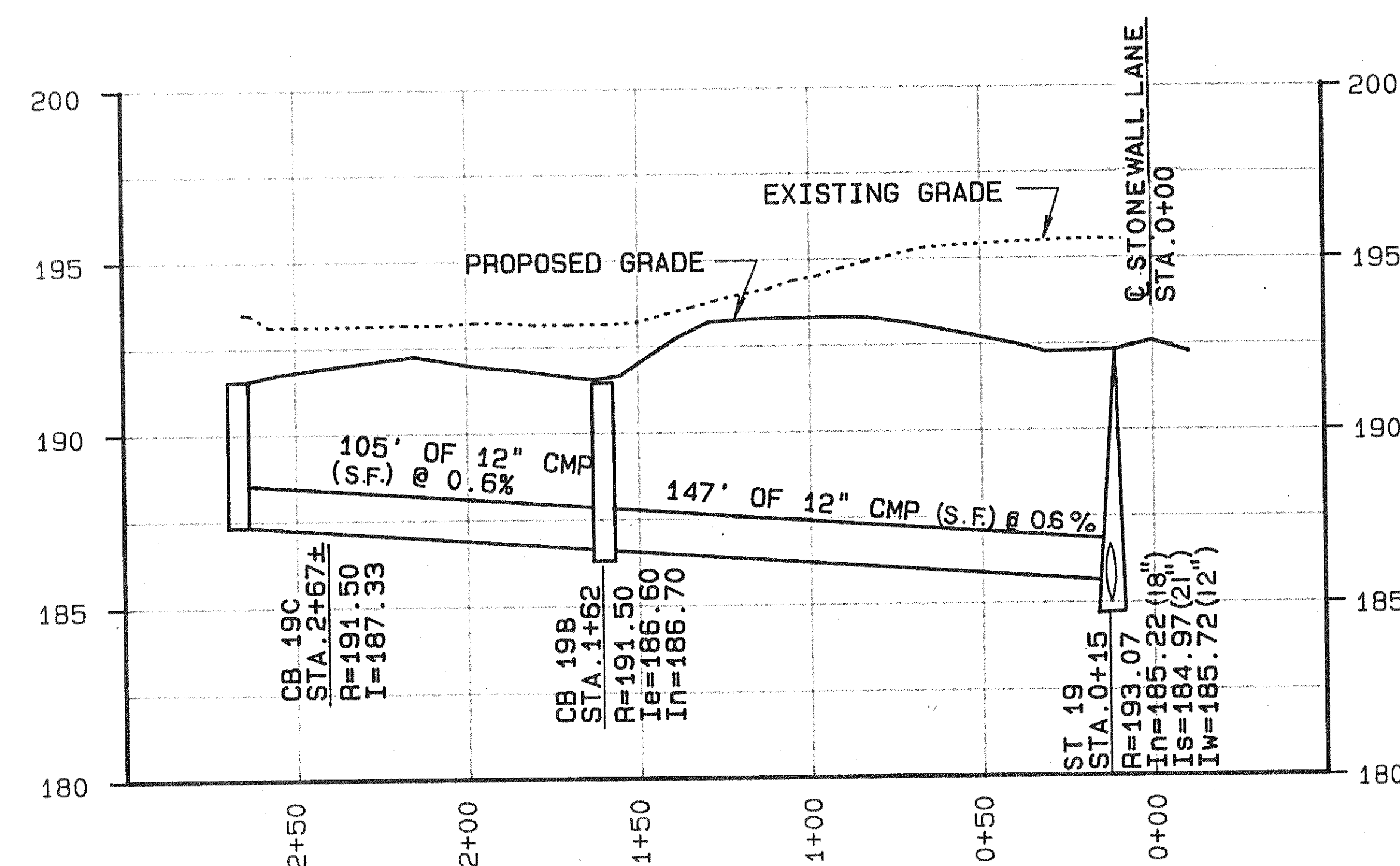
PROFILE-SOUTH WINDSOR COURT DRAINAGE SCALE: HORIZ. 1"=50' VERT. 1"=5'
