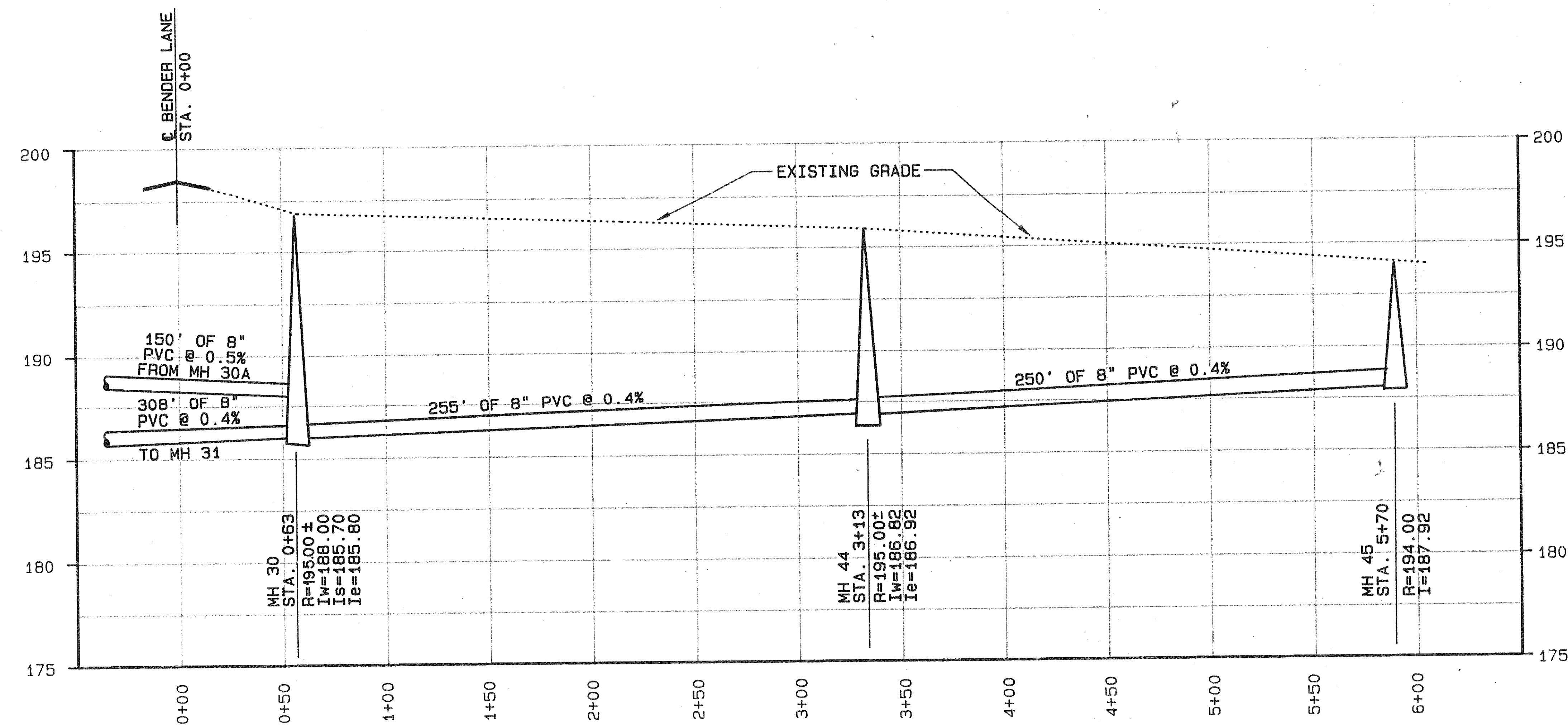
PROFILE-UPPER LOTS SANITARY SEWER SCALE: HORIZ. 1"=50' VERT. 1"=5'
