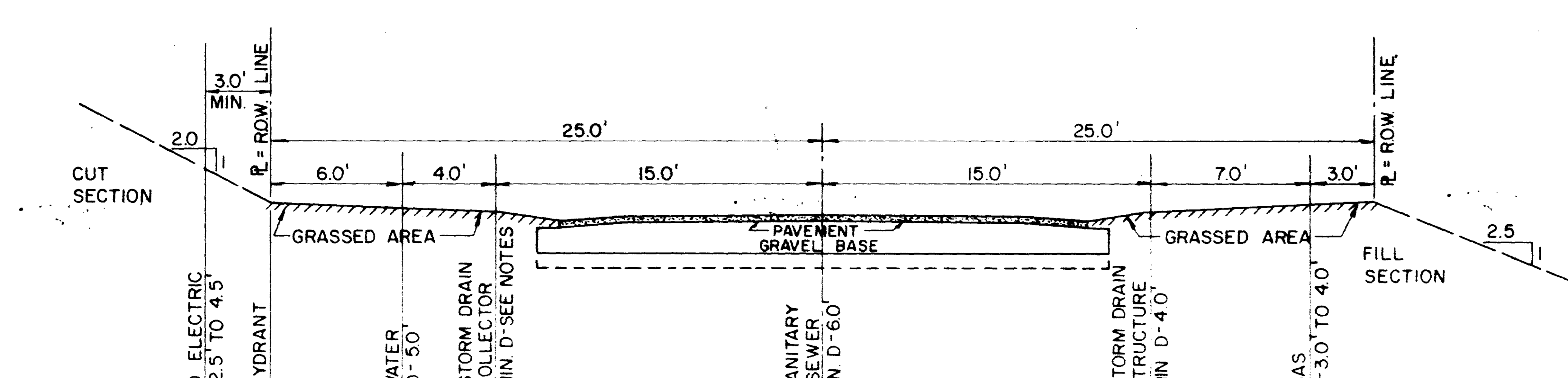
ROW WIDTH = 50 FT. TYPICAL SECTIONS NORMAL LOCATIONS FOR UNDERGROUND UTILITIES & FACILITIES (SCALE: 1" = 5'-0")
