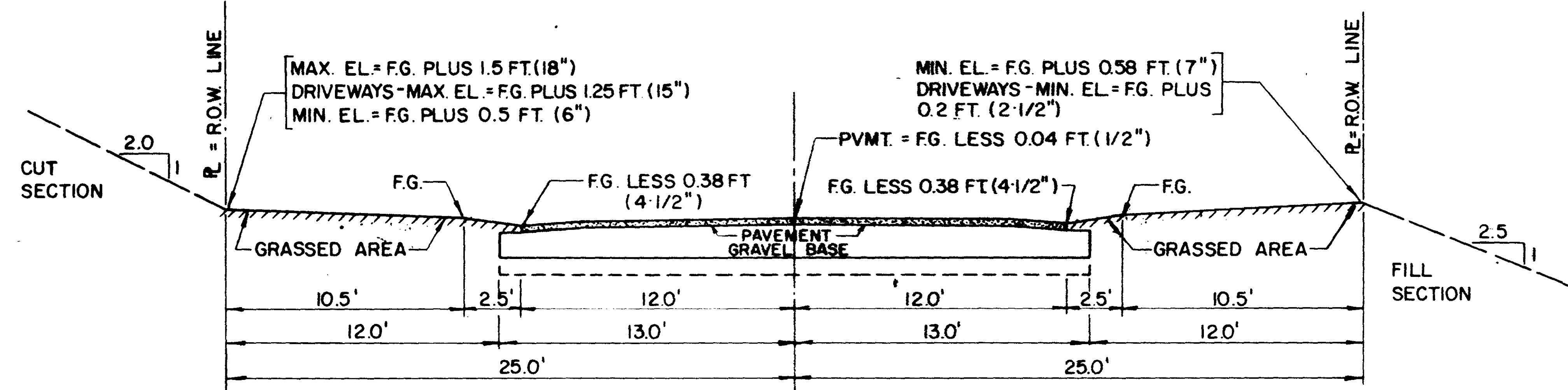
ROW WIDTH = 50 FT. TYPICAL SECTIONS CROSS SECTION UPON FINAL COMPLETION OF HIGHWAY (SCALE: 1" = 5'-0")
